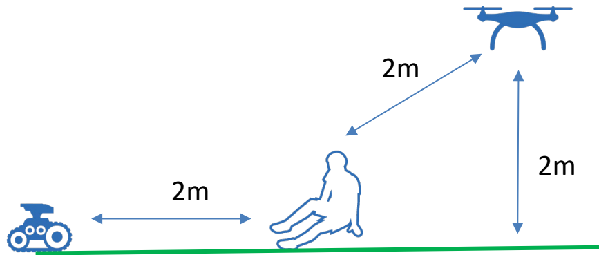
Figure 8a: Standoff Distance. The standoff distance is measured from UxS to ground or nearest body part to nearest UxS part.
