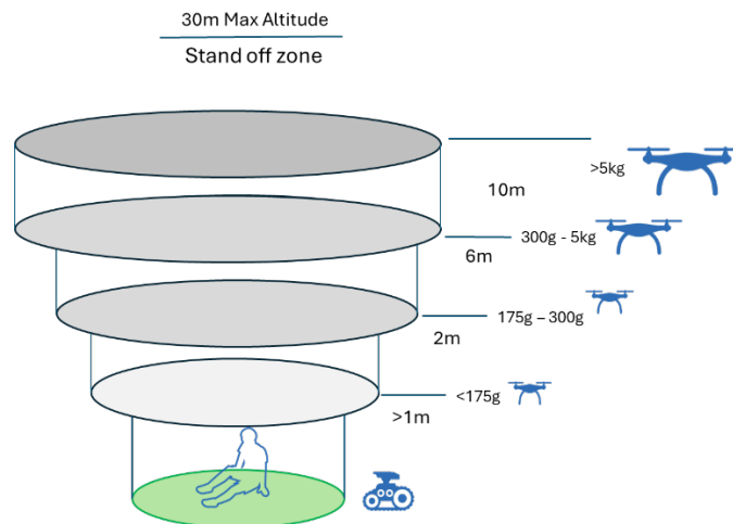
Figure 8b: Size-based standoff distances: Standoff distance is a hemisphere with a minimum height from the ground based on UAS size. The UAS may not hover in a 1m cone directly over the casualty.
