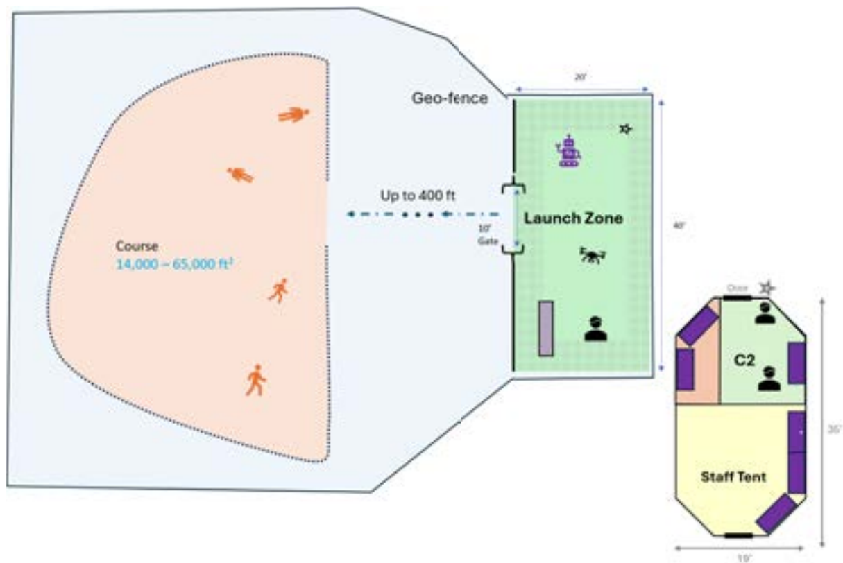
Figure 5b: Team staging area for HMT lanes may not be co-located with the course. The MCI will consist of a smaller unmarked area within a larger geofence.
