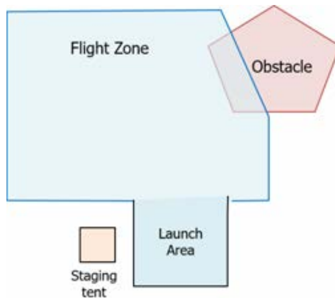
Figure 6: Flight zone around the course will be unmarked, teams must rely on geofences, the GPS coordinates will be provided. The flight zone may contain large obstacles including trees, vehicles and buildings, teams should maintain awareness of drone location.
