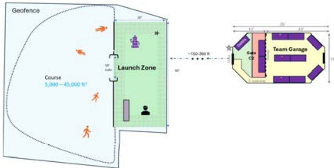
Figure 5a: Team Staging Area for Gates. The launch zone will be separated from the course by a wall with a 10' wide gate in the wall. The location of the launch zone will be separated from the C2, which will be located in team garages.
