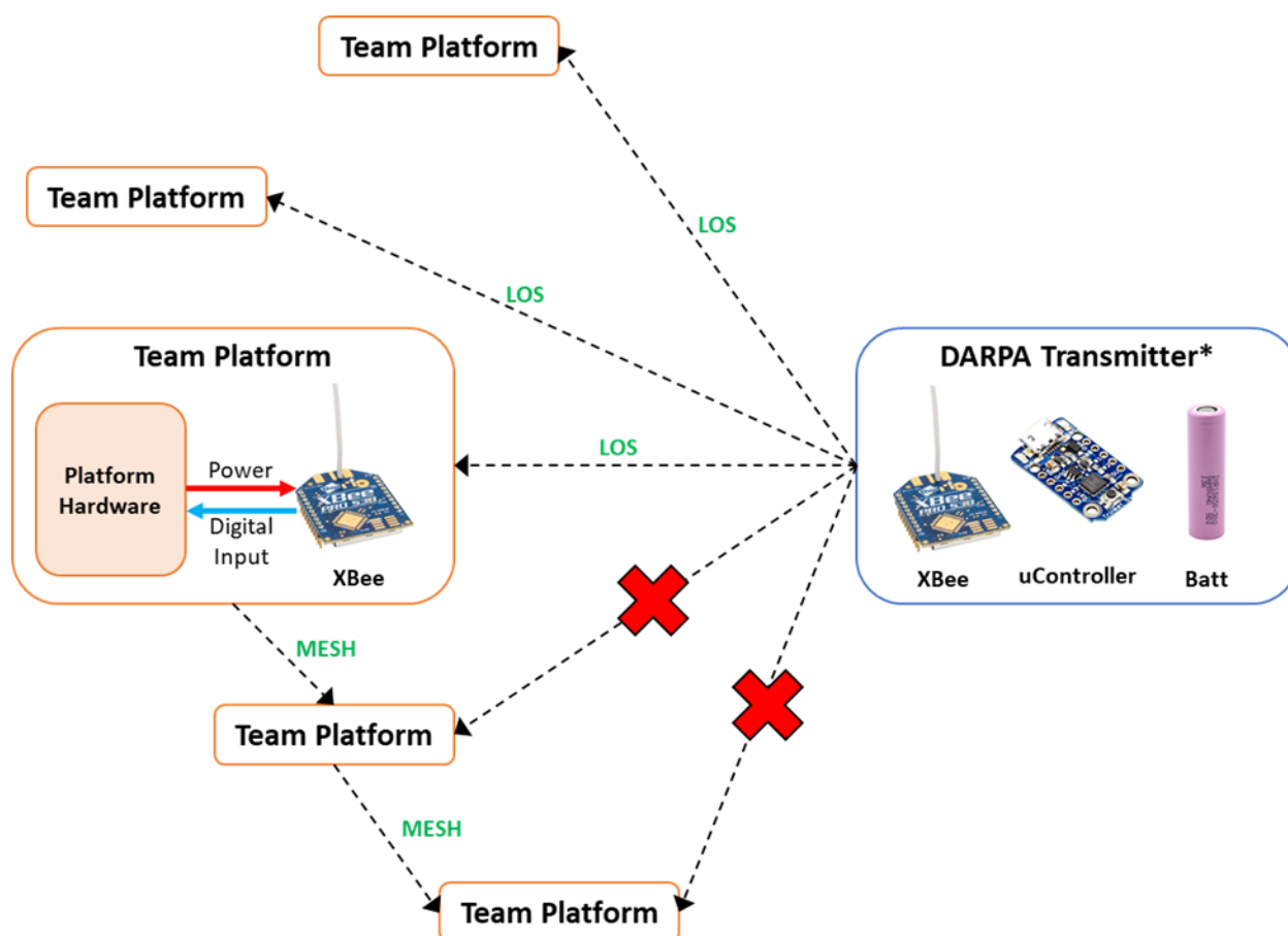
Figure 1: Concept of Operations for the Recovery Wireless E-Stop System
